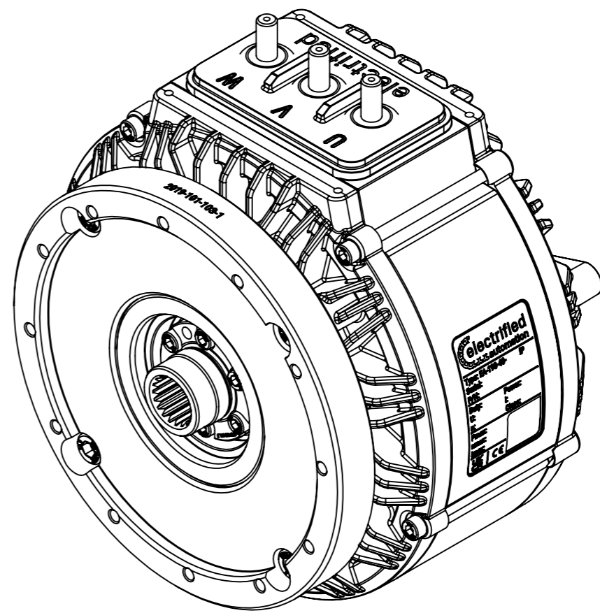
ISOMETRIC VIEW
