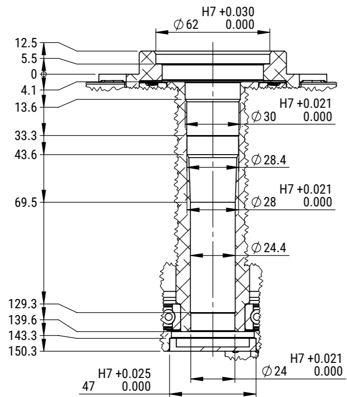
SECTION B-B (CROPPED)
