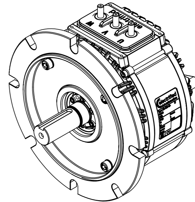
ISOMETRIC VIEW
