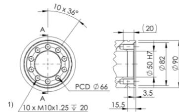
Shaft end
